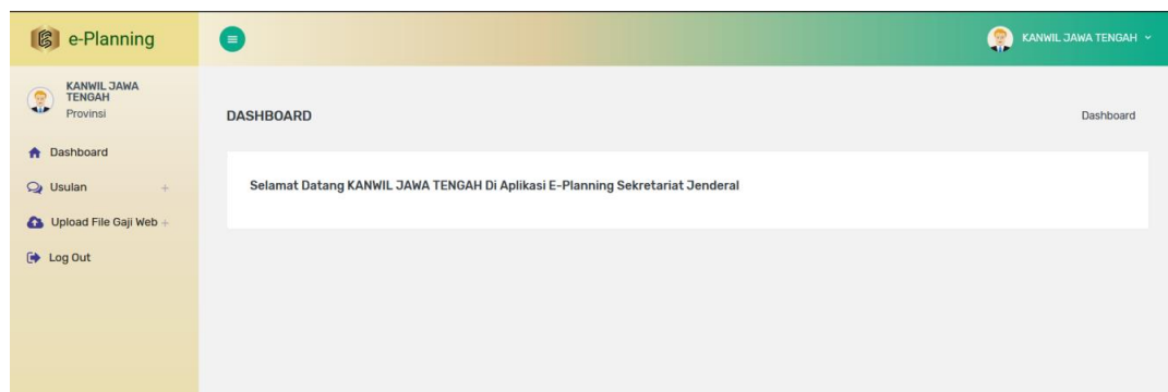
Gambar 61 Dashboard
