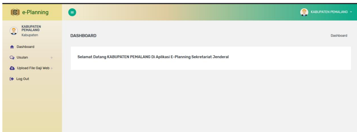
Gambar 3 Menu Awal/Dashboard
