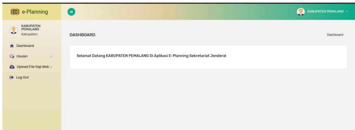
Gambar 4 Dashboard Satker
