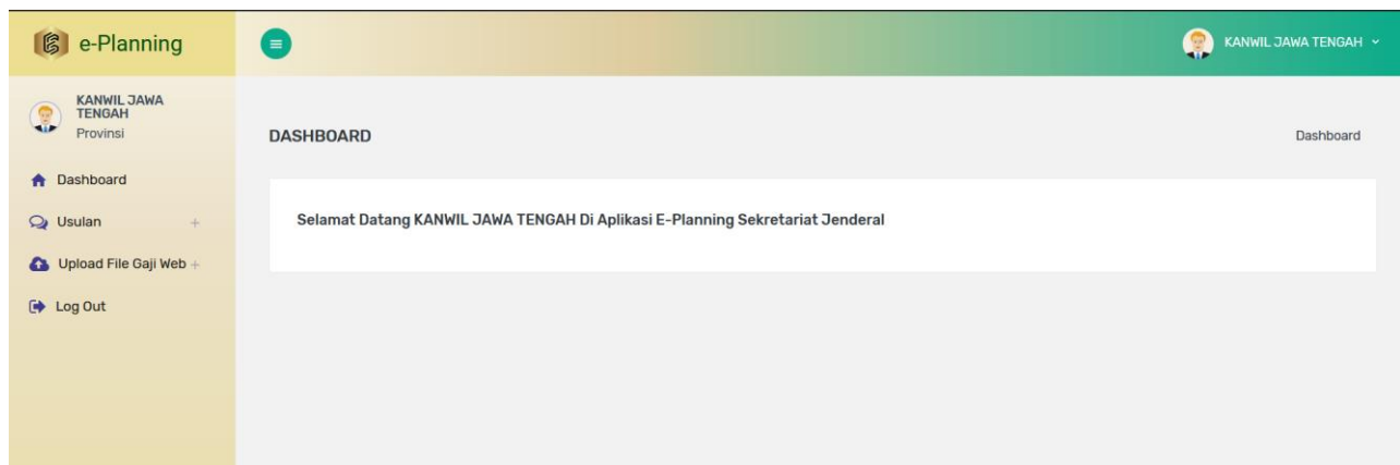
Gambar 60 Menu Awal/Dashboard
